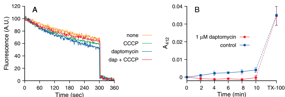
Fig. 4. Absence of liposome permeabilization toward chloride (A) and cysteine (B). A: Pyranine-loaded liposomes with an interior pH of 6 were diluted with 100 mM choline chloride, pH 8, and CCCP (5 nM) and daptomycin (1 \mu\text{M} ) were added at t = 0 . Permeabilization for chloride should have resulted in an accelerated dissipation of the pH gradient and concomitant drop in pyranine fluorescence. The experiment shown is one of 4 independent ones and is a representative. B: Time course of the reduction of DTNB entrapped in liposomes by 100 mM cysteine added to the outside, in the absence and presence of daptomycin (1 \mu\text{M} ). Reduction of DTNB results in an increase of the absorption at 412 nm. After the last reading at 10 min, samples were solubilized with Triton-X100, resulting in immediate complete DTNB reduction. Error bars are standard deviations from three independent experiments. Daptomycin does not increase in the permeation of cysteine into the liposomes.
