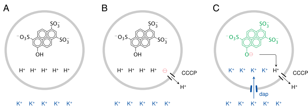
Fig. 2. Schematic representation of the pyranine-based liposome permeabilization assay, using \text{K}^+ ions as an example. Liposomes loaded with pyranine were diluted into the final reaction buffer to create two opposite ion concentration gradients across the membrane (A). Application of the protonophore CCCP alone will create a diffusion potential, which will prevent a major efflux of protons (B). If daptomycin is added also and allows \text{K}^+ ions to enter, both ion gradients can dissipate, the pH in the liposome will rise, and pyranine fluorescence will increase (C).
