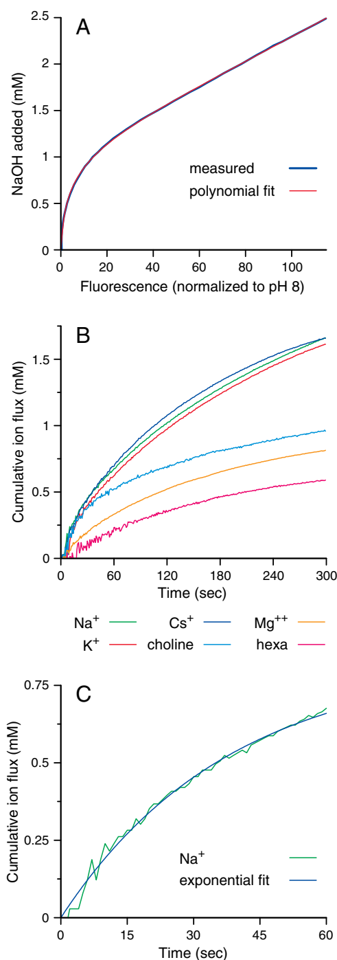
Fig. 5. Conversion of observed pyranine fluorescence changes to cation flow rates. A calibration curve relating total (buffered and unbuffered) proton concentration to pyranine fluorescence intensity was obtained by titrating a solution matching the liposome interior with NaOH (A). A polynomial function was fitted to the measured values. In panel B, the polynomial function obtained in A was applied to the raw fluorescence traces shown in Fig. 3C in order to transform them to ion fluxes. The flow rates for hexamethonium and Mg^{++} were then divided by 2, as each of these cations is exchanged for 2 protons. In C, an exponential function was fitted to the transport curve for sodium in order to estimate the initial transport rate (see text for further details).
