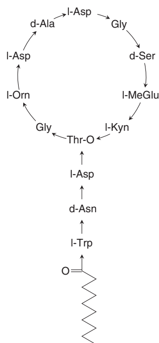
Fig. 1. Schematic of the structure of daptomycin. Arrows indicate amide bonds, except between kynurenine and threonine, where an ester bond between the carboxyl group of kynurenine and the side chain hydroxyl group of threonine closes the ring.
