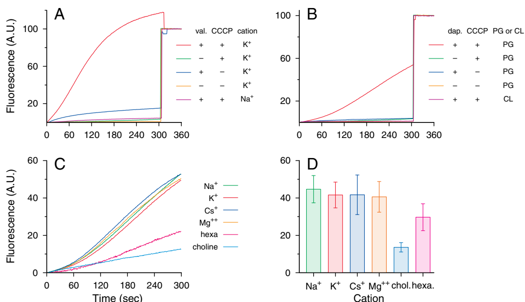
Fig. 3. Time-based fluorescence traces of pyranine-loaded liposomes after exposure to different test solutes and permeabilizing agents, which were added at t = 0 . The interior pH was 6 and the exterior pH was 8. Test solutes added to the exterior buffer at 100 mM were KCl in B, and otherwise as indicated; “hexa” in C and D is hexamethonium. After 300 s, the samples were solubilized with Triton-X100, and the fluorescence monitored for another minute. The fluorescence intensity observed after Triton solubilization was used to normalize each fluorescence trace. A: Valinomycin (val., 0.5 \mu\text{M} ) with CCCP (5 nM) permeabilizes liposomes for potassium but not sodium. B: Daptomycin (1 \mu\text{M} ) plus CCCP (5 nM) also causes permeabilization for potassium of membranes containing PG, but not cardiolipin. C: Permeabilization traces obtained with both daptomycin and CCCP present, after subtraction of the traces obtained with CCCP only. D: Averages and standard deviations of fluorescence intensities after 300 s of incubation, for 3 or 4 independent experiments performed as in C (“chol.” is choline).
